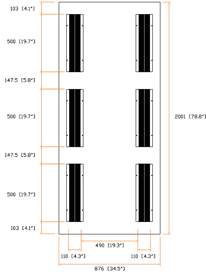
Front view :
