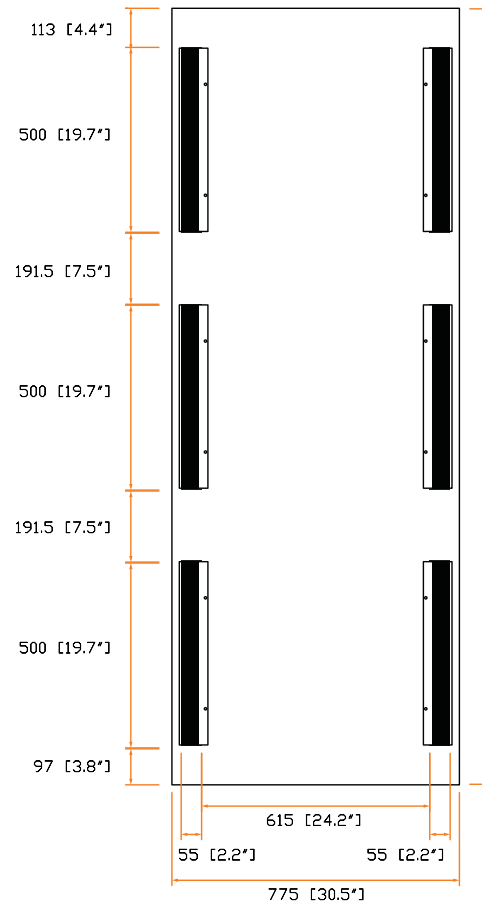
Front view :
