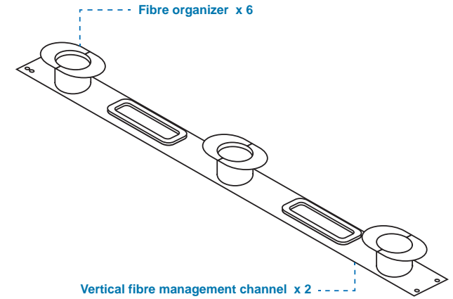
Vertical fibre management channel x 2
